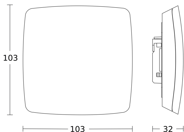
Dimension Drawing 1
